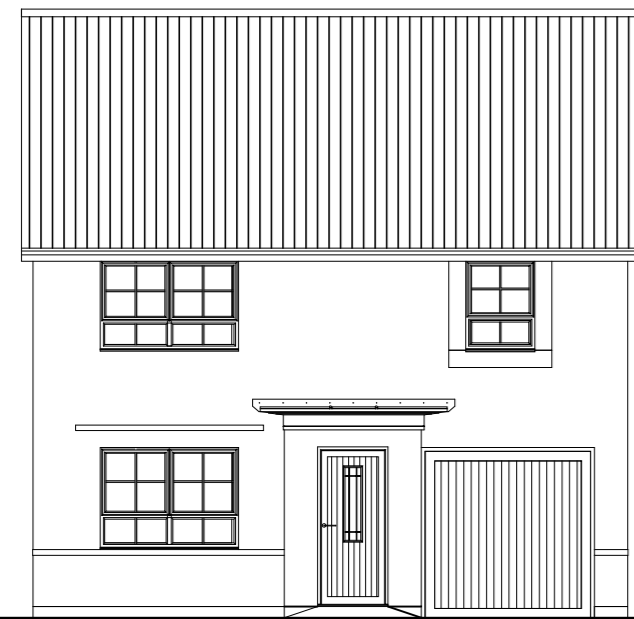
FRONT ELEVATION
