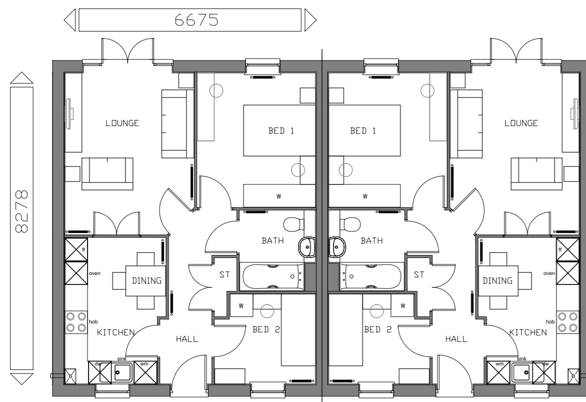
FLOOR PLAN
