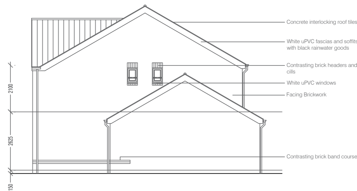
Side Elevation
